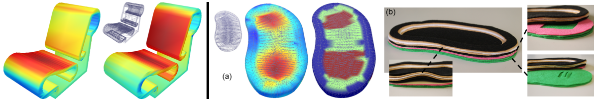
Fig. 7. Applications. Left: Personalized Softness Metrics. An input chair model and two different softness maps from two different users. Right: Fabrication Example. (a) An input 3D model of the bottom part of a sandal, the softness map computed by our method, and the softness values discretized into three types for fabrication purposes. (b) The sandal fabricated with layers of felt material. We also show (small inset images) some simple ways we experimented with to adjust the softness (e.g. adding a harder card piece, cutting a hole, or stripes of holes) if we were to press top-down into the object to match the values our method computed.
